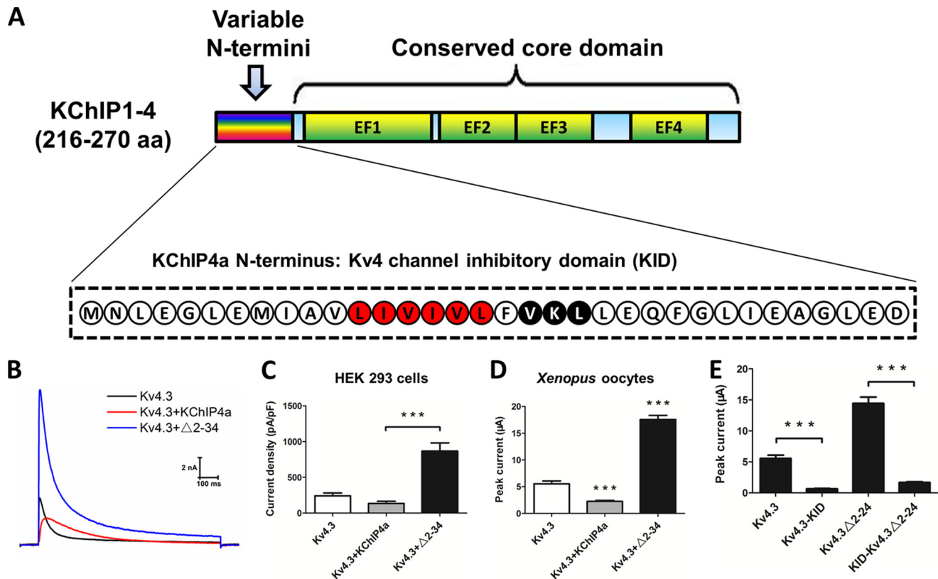
FIGURE 1. The N-terminal KID of KChIP4a suppresses Kv4.3 function. A , a schematic representation of the general domain structure of KChIPs. KChIPs consist of an NH 2 -terminal variable domain ( multicolored box ) and a conserved COOH-terminal core domain ( light blue boxes ) containing four EF-hands ( light green boxes ). The N-terminal domain of KChIP4a (designated KID in this study) is represented with the single-letter amino acid code in the protein sequence. The LIVIVL motif is marked in red , and the VKL motif is marked in black . B , representative current traces of Kv4.3 alone, Kv4.3-KChIP4a, and Kv4.3-KChIP4a \Delta 2-34 recorded from HEK 293 cells. The currents were evoked by a 1-s depolarizing pulse to +40 mV from a holding potential of -100 mV. C , quantitative analysis of peak current densities recorded from HEK 293 cells expressing the indicated channels or channel complexes. Values are mean \pm S.E. ( error bars ); n = 6-10 cells; ***, p < 0.001 . D , quantitative analysis of peak current amplitudes recorded from Xenopus oocytes expressing the indicated channels or channel complexes. Values are mean \pm S.E.; n = 10-26 oocytes; ***, p < 0.001 . E , the fusion of the KID to the C-terminal end of Kv4.3 (Kv4.3-KID) or the N terminus of Kv4.3 N-terminal truncation mutant (KID-Kv4.3 \Delta 2-24) significantly suppressed the channel current. Values are mean \pm S.E.; n = 5-10 oocytes. Statistical significance was assessed using Student's t test, and statistical significance was considered as p < 0.001 (***)
